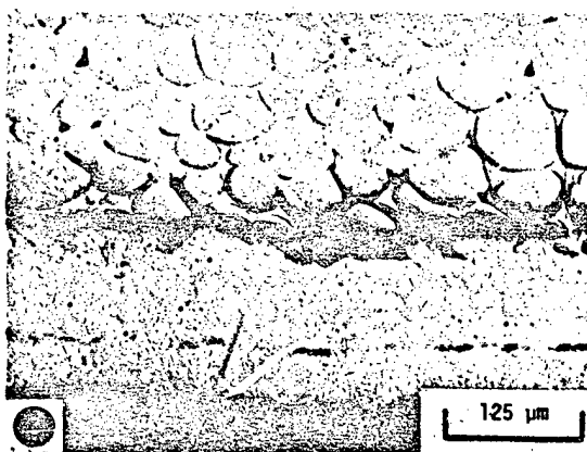
Fig. 1. Representative microstructures of the composite--copper junction showing bonding.
