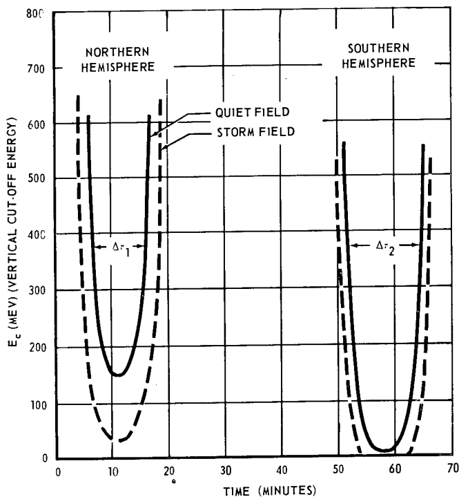
Figure II-11. Variation of magnetic cut-off energy with time for first orbit [60° inclination and 200-n.m. (~400-km) altitude].
