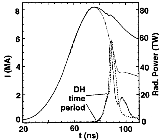
Figure 9. Comparison of experimental (solid, dotted) and simulation (dot-dash, dashed) currents and radiation powers for a Saturn dynamic hohlraum (DH) experiment. The time period when the dynamic hohlraum exists (the "foot" of the radiation pulse) is marked. The tungsten implosion portion of the calculation is the same as that for Fig. 3.
